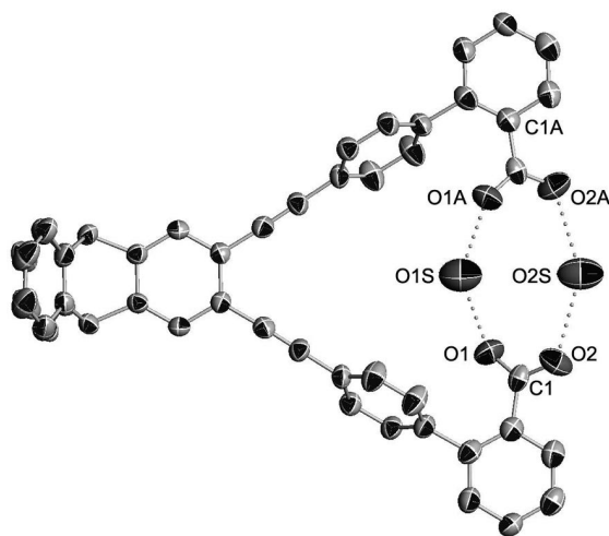
Figure 5. Molecular structure of 4b and two co-crystallized water molecules at 100% and 50% occupancy for O2S and O1S, respectively, with strong hydrogen bonding (dotted line) between the carboxylic acid and the solvent. Thermal ellipsoids are drawn at the 50% probability level. Hydrogen atoms, exo -oriented disordered carboxylic acid moieties at 33% occupancy, two water molecules (both 25% occupancy), and two methanol solvent molecules (both 25% occupancy) are omitted for clarity.
