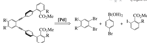
Scheme 1. Synthetic route to C-clamp ligands; R = H or Ph and \text{R}'_2\text{C}_6\text{H}_2 = triptycene or veratrole backbone.
