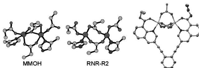
Figure 1. The reduced diiron(II) MMOH (left) and RNR-R2 (center) cores and a diiron(II) model complex [\text{Fe}_2(\text{Et}_2\text{BCQEB}^{\text{Et}})(\mu\text{-O}_2\text{CAr}^{\text{Tol}})_3]^+ (right) displaying the N-donors in a syn disposition with respect to the iron–iron vector. The location of the atoms is based on X-ray coordinates. The ethyl moieties on the phenyl ring, and the aromatic carbon atoms of the – O 2 CAr Tol ligands (except the \alpha -carbon atoms) are omitted for clarity in the model compound.
