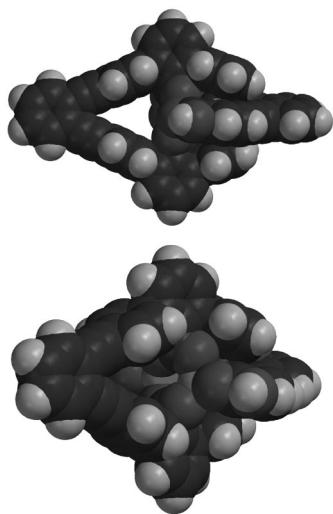
Figure 2. The energy-minimized structure [14] of [\text{Fe}_2\{\text{DEV}-(\text{PICMe})_2\}\{\text{DEV}(\text{terphCO}_2)_2\}] displaying the substrate-access cavity (top) and the exposed diiron center (bottom).
