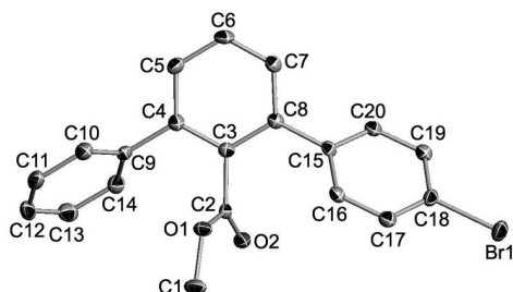
Figure 4. Molecular structure of 3 . Thermal ellipsoids are drawn at 50% probability level. Hydrogen atoms are omitted for clarity.
