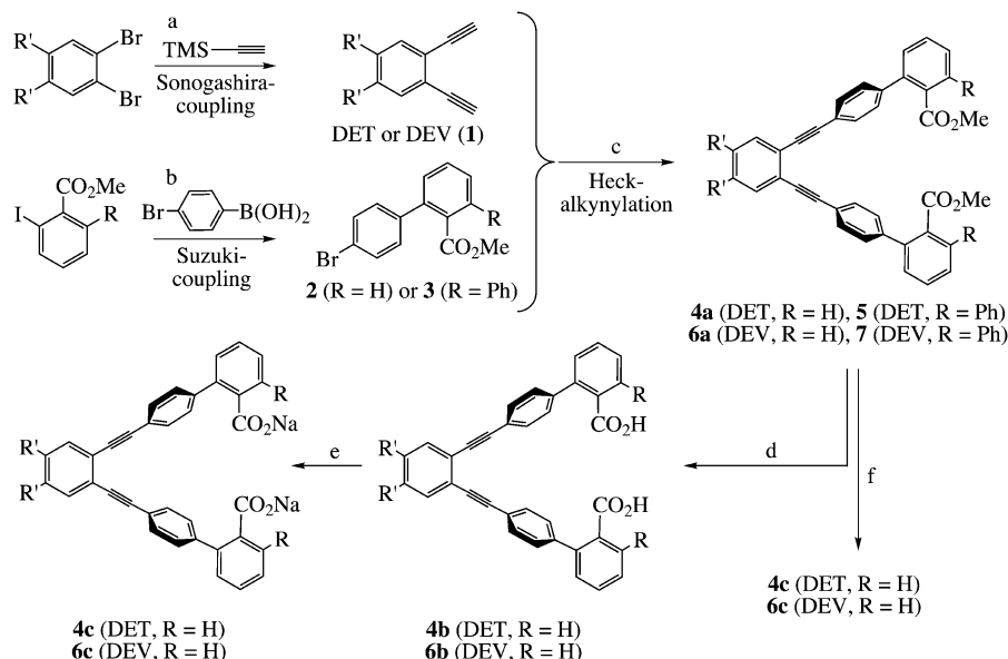
Scheme 2. Synthetic pathway to diethynylbenzene-based C-clamp ligands; R'_2C_6H_2 = triptycene or veratrole backbone. (a) 2 steps, 1: [Pd(PPh_3)_4]/CuI , piperidine, 100 °C; 2: K_2CO_3 , MeOH, ref. [12] ; (b) [PdCl_2(PPh_3)_2] , 1 M Na_2CO_3 , THF, 60 °C; (c) [Pd(PPh_3)_4] , Et_3N , THF, 70 °C; (d) LiI , pyridine, 110 °C; (e) NaOH , MeOH, 60 °C; (f) NaOTMS , THF, 60 °C.
