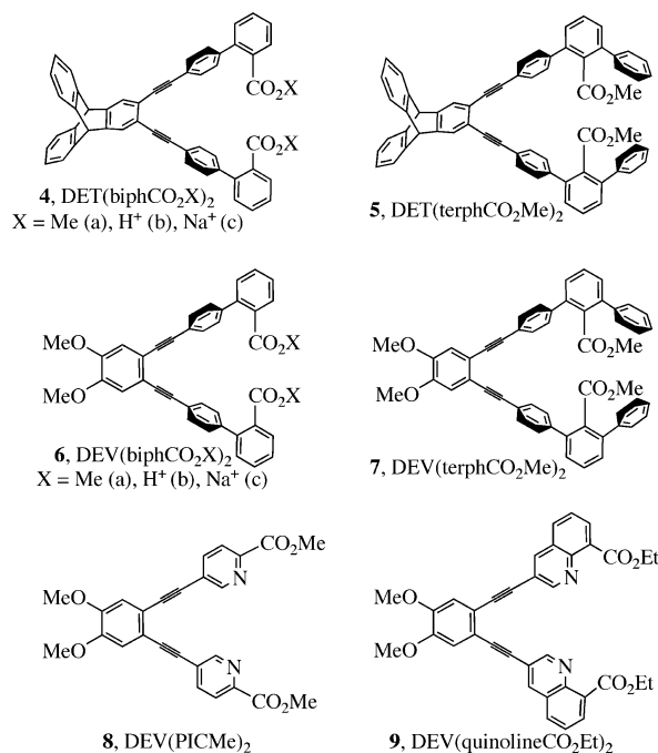
Figure 3. Graphic representation of the C-clamp ( 4–7 ) and syn -N-donor ( 8 and 9 ) ligands.
